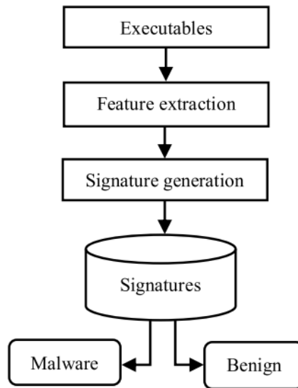
Figure 4: signature-based malware detection schemas
